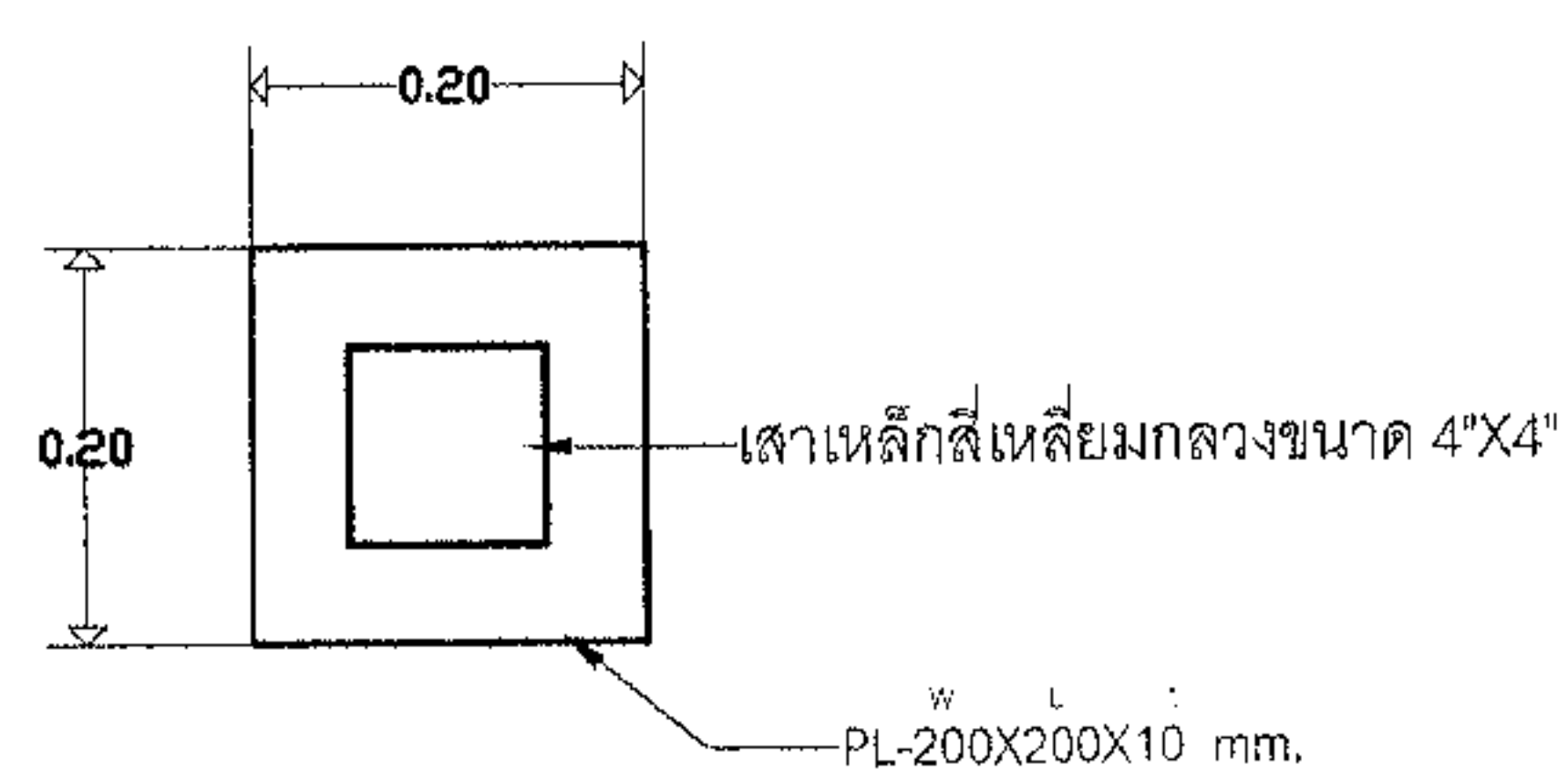
JOINT "FIXED" DETAILS SCALE 1: 15
