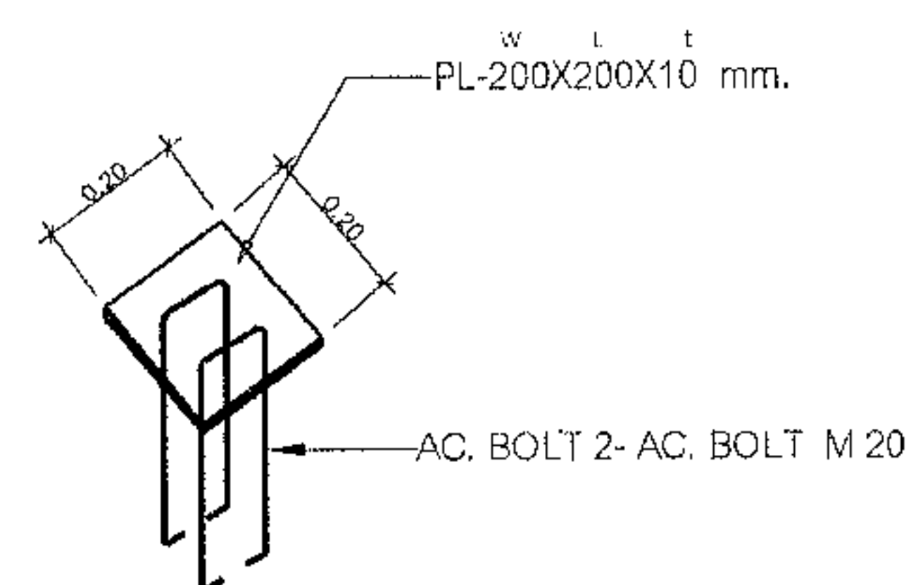
STEEL PALTE DETAIL
