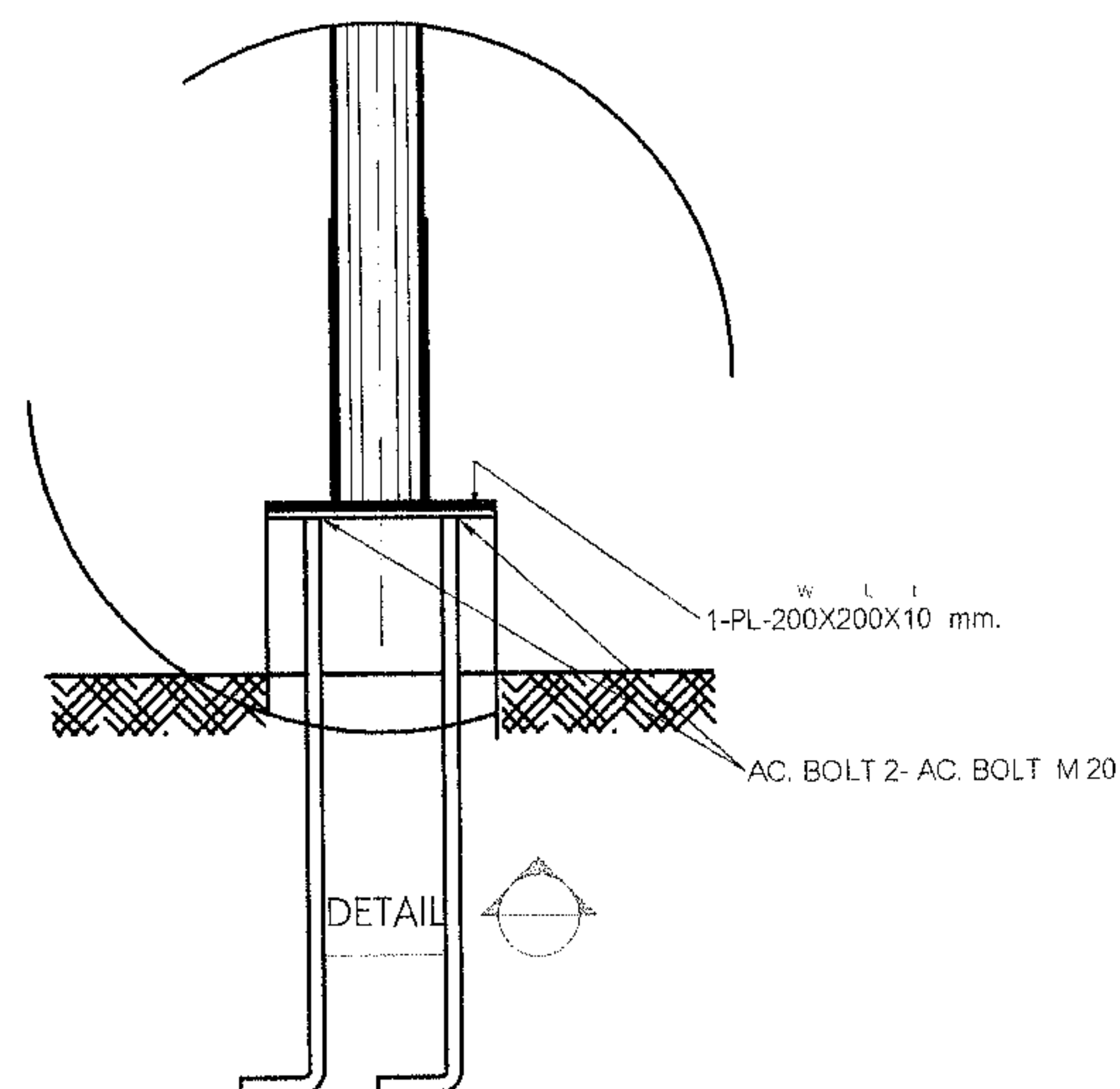
AC. BOLT DETAIL SCALE 1: 15
